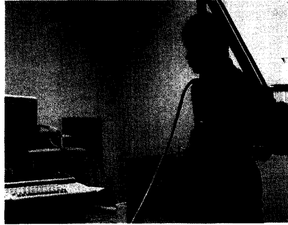
Figure 4: Experimental setup. The 2DE scanner, whose linear scanhead mounted on the mechanical tracking arm, and a phantom in the watertank is seen.
