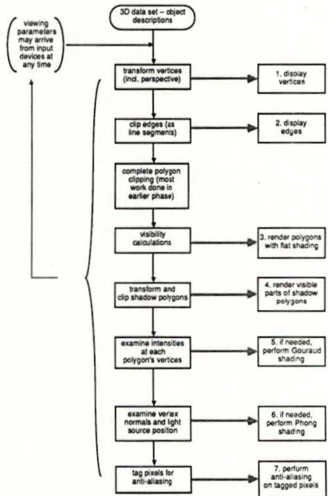
Figure 2: Rendering pipeline modified for adaptive refinement
