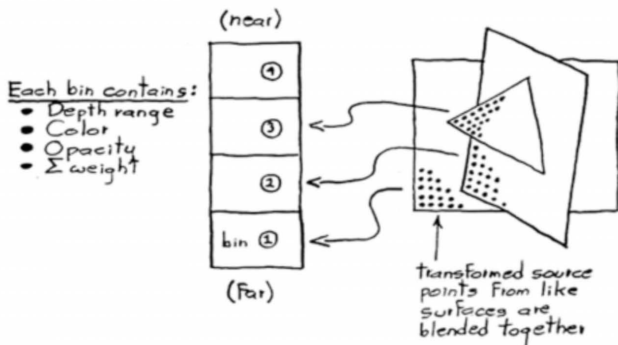
Figure 4a: Blending calculations
