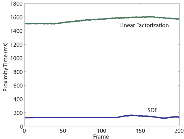
Figure 8: Timing comparison between our algorithm and a GPU-based volumetric distance field algorithm [SGGM06] labeled as SDF and Linear Factorization respectively: Our algorithm is able to achieve 5–10 times speedup in proximity computation between two deforming alphabets. The scene is composed of 3.7K polygons. The surface distance field is computed at a resolution of 512 \times 512 and the volumetric distance field is computed at 180 \times 150 \times 256 . Our algorithm is able to obtain higher accuracy in distance field computation on the surface and achieves an interactive performance of 5–10 frames per second.
