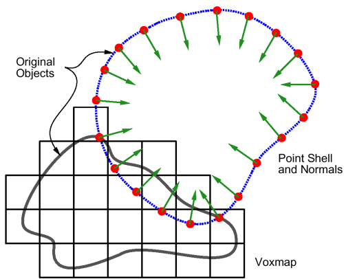
Figure 3: A point shell colliding with a voxmap (figure from [McNeely99]).
