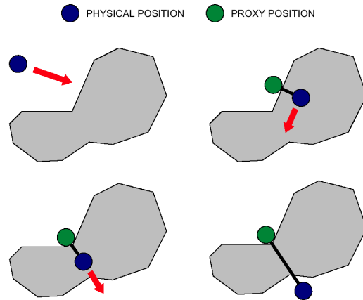
Figure 2: Virtual proxy example (figure from [Ruspini97])
